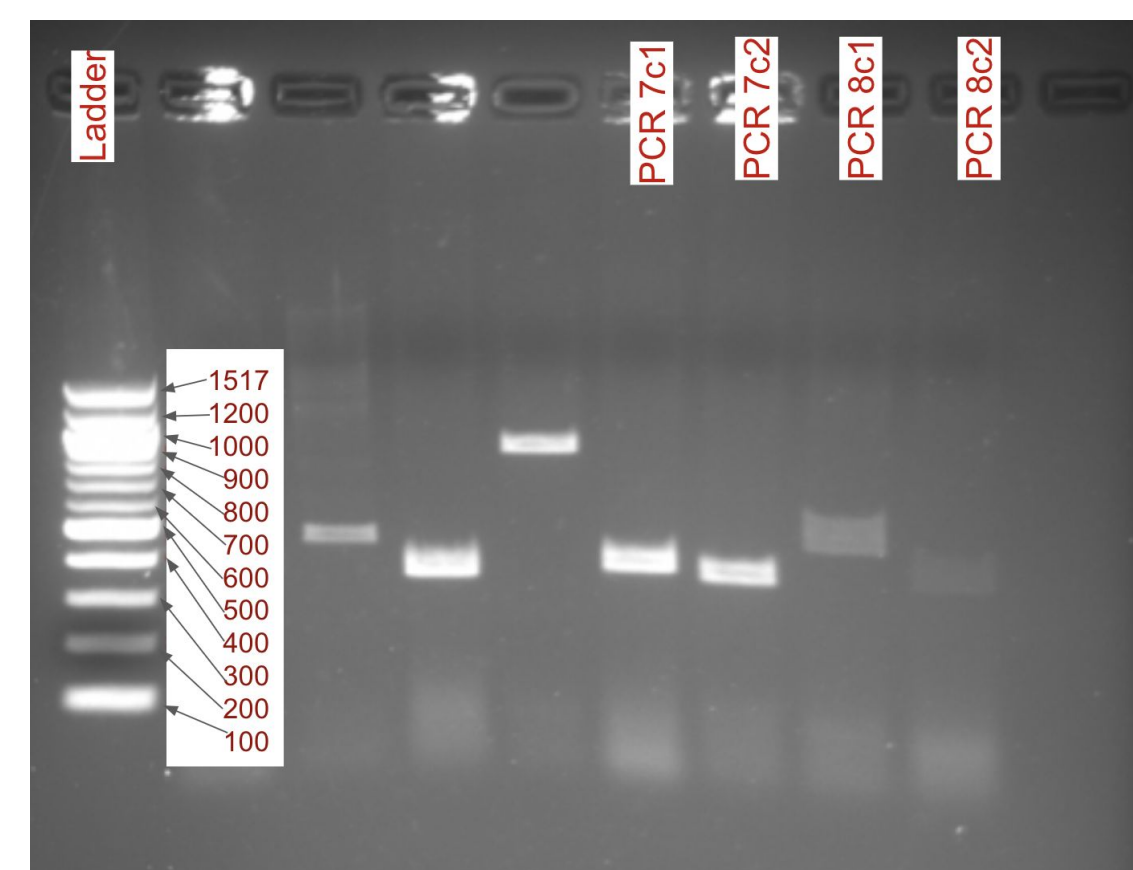
Figure 1. Gel Electrophoresis.
