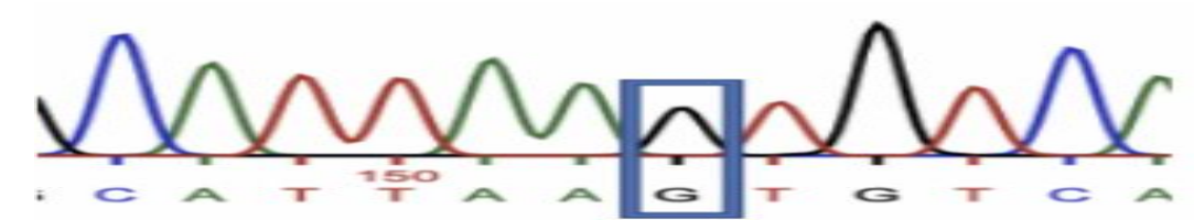
Figure 5. SNPBH Chromatogram.
