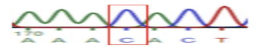
Figure 3. SNP2 Chromatogram.
